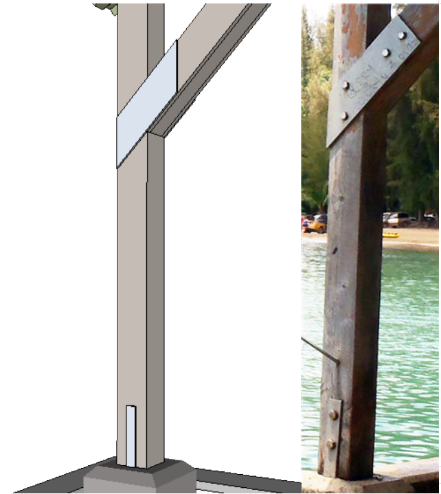
knee brace bracket, top
